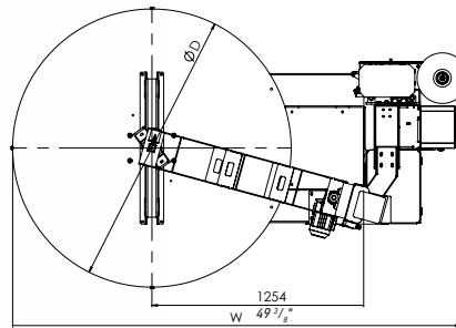
PRE-STRETCH SYSTEM
